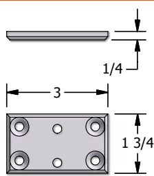
FL6.2 SURFACE-MOUNT
