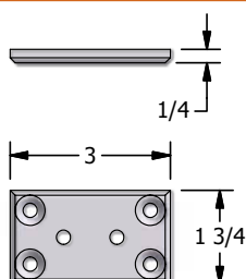
FL6.1 SURFACE-MOUNT
