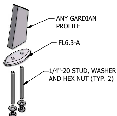
DETAIL VIEW OF CONCEAL MOUNT ASSEMBLY
