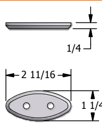
FL6.3 CONCEALED-MOUNT
