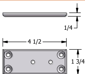
FL6.5 SURFACE-MOUNT FOR VGG1.3 ONLY
