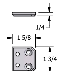
FL6.4 END PANEL SUPPORT FLANGE
