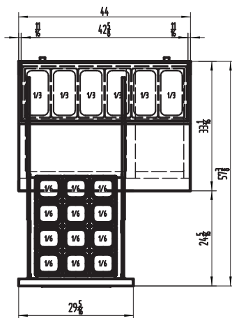
C-PP44-D-HC TOP VIEW
