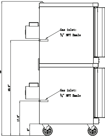
SIDE VIEW - DOUBLE
