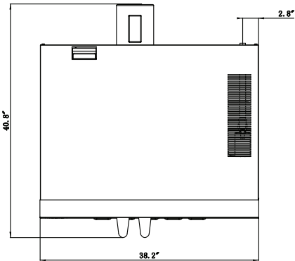
TOP VIEW C-CO1-SD-NG and C-CO1-SD-LP
