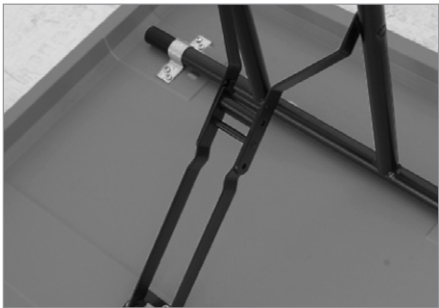
Spring-loaded, leg-brace locking mechanism.
