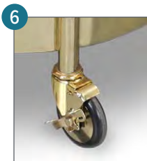
4" Brass plated casters (two with brakes)
