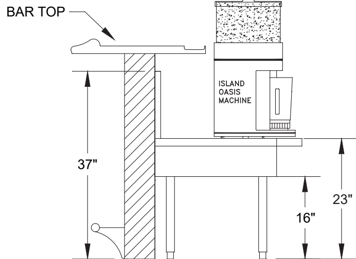
Installation Side Elevation
