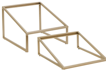
Angled Riser Pivot Champagne 7364MW341 L 13 7/8" W 11 1/2" H 8 1/2" CP 1 7364MW342 L 13 7/8" W 11 1/2" H 4 1/2" CP 1
